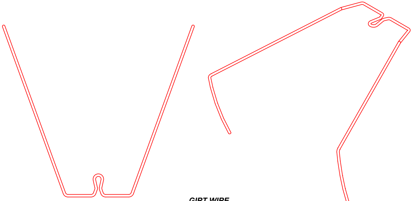
GIRT WIRE (GW-X) X = WIRE SIZE
